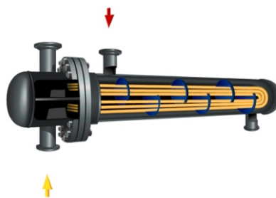
U-Tube-Heat-Exchanger
